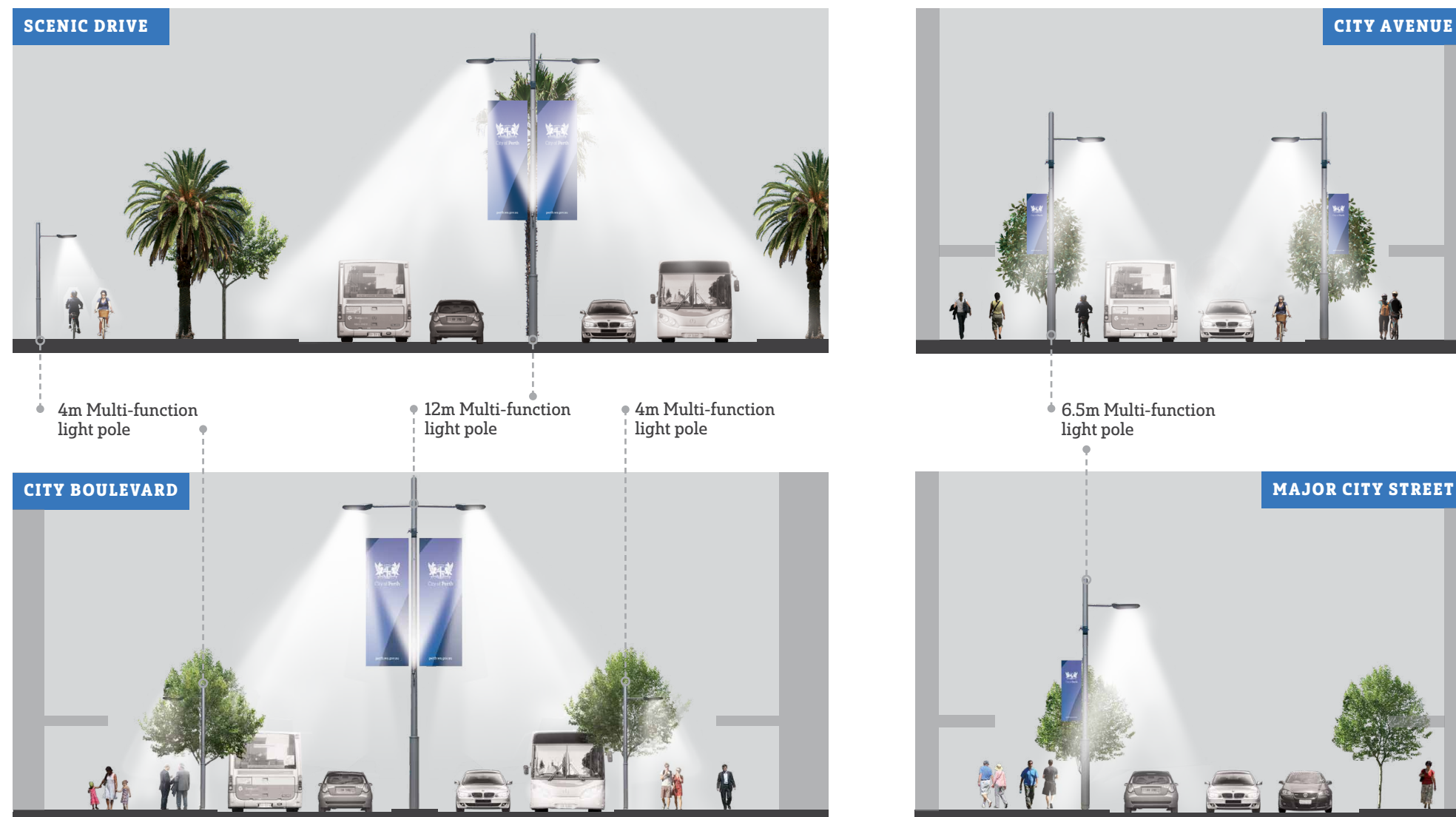
FIGURE 12: STREET LIGHTING ARRANGEMENT
